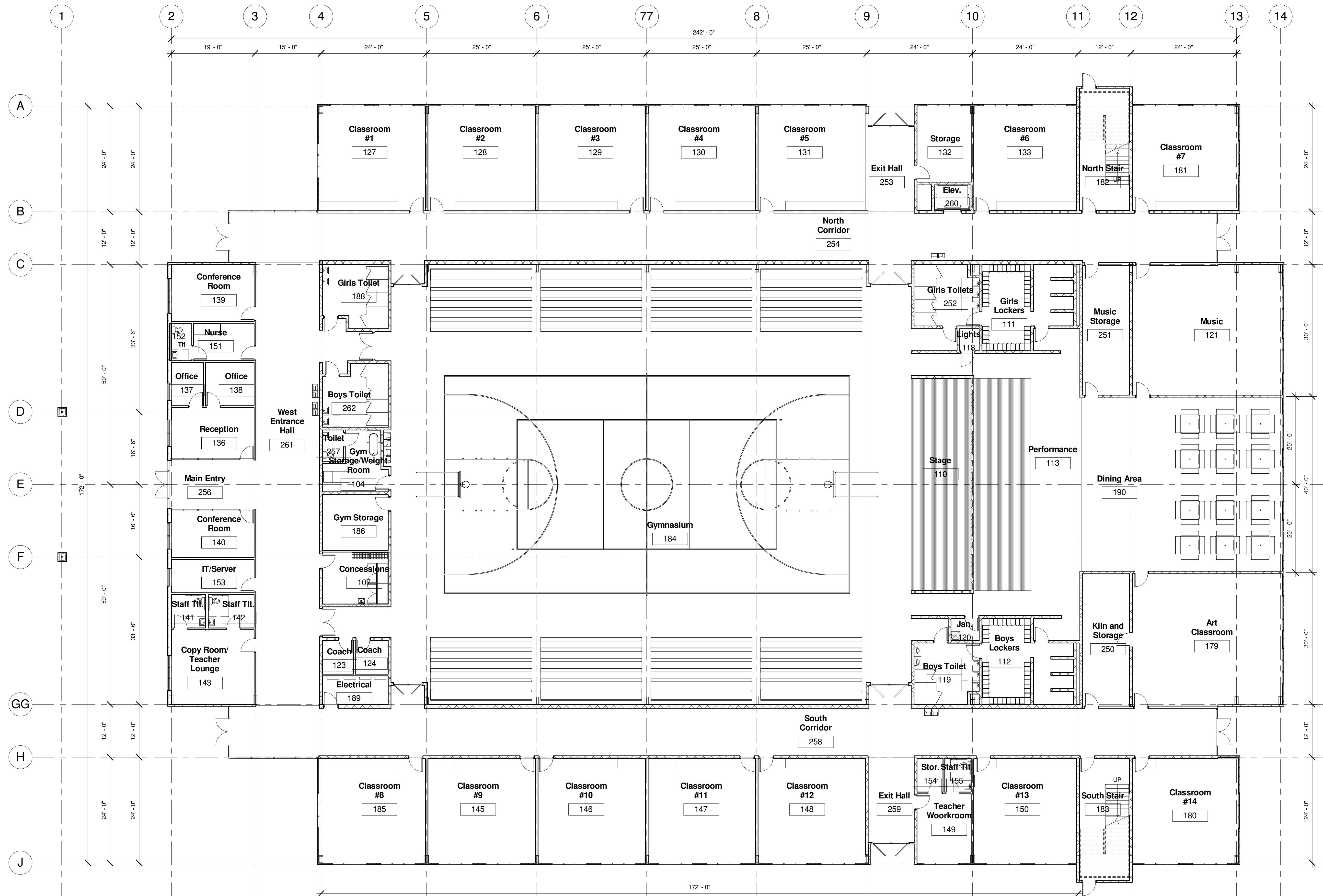
1 First Floor Plan - Elementary School AREA: 41,131 SF 3/32" = 1'-0"
